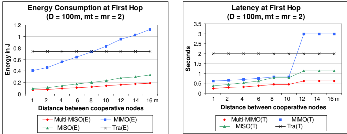
Figure 5: Energy consumption and latency at the first hop, when mt = mr = 2 , D = 100\text{m} , and d changes from 1m to 16m
